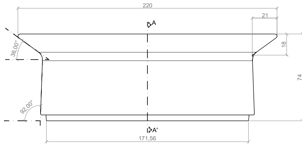
ALZADO / FRONT VIEW
