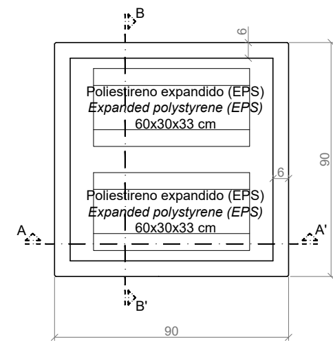
VISTA INFERIOR / BOTTOM VIEW
