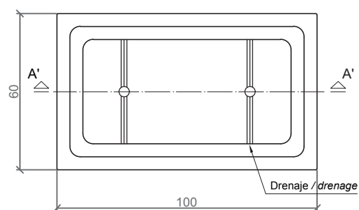
VISTA INFERIOR / BOTTOM VIEW
