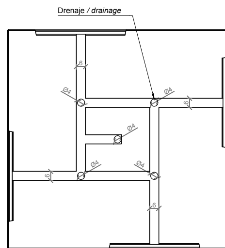
VISTA INFERIOR / BOTTOM VIEW
