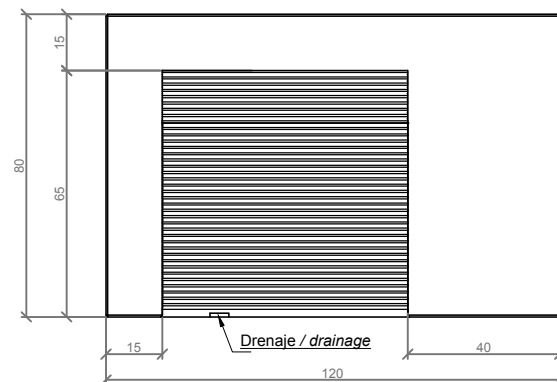
ALZADO / FRONT VIEW
