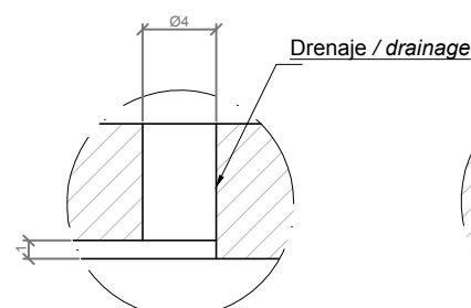
DETALLE M / DETAIL M
