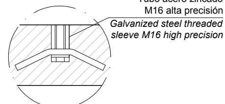
DETALLE C / DETAIL C
