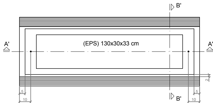
VISTA INFERIOR / BOTTOM VIEW
