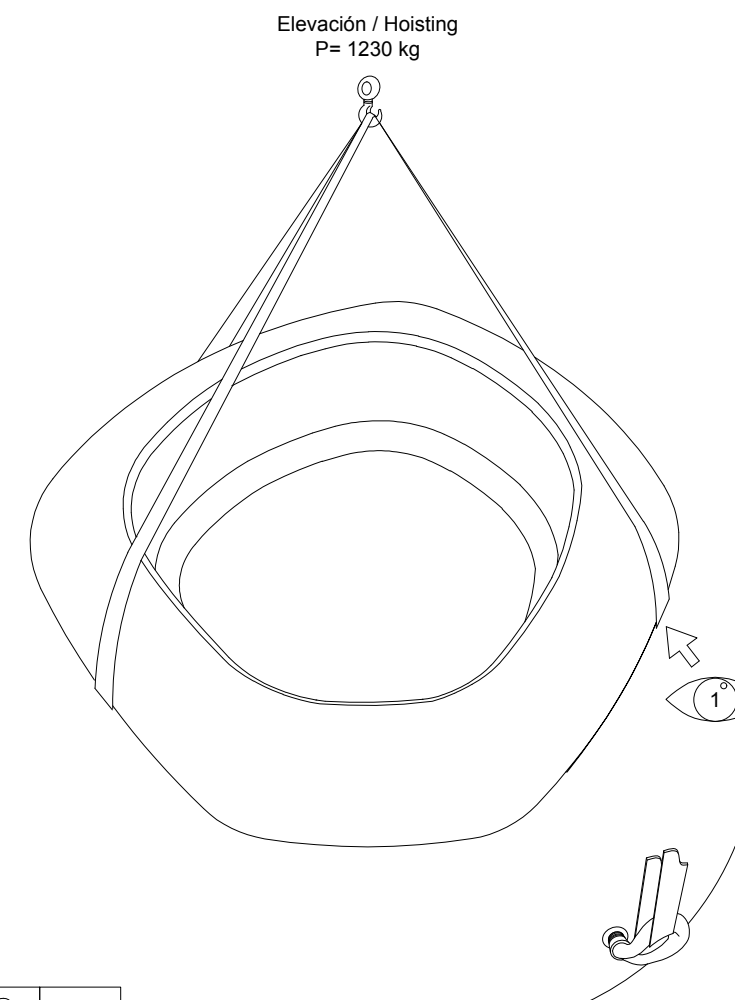
DETALLE 1 / DETAIL 1
